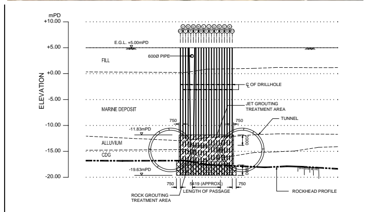
Triangular Grid 1m x 1m Column Diameter 1.5m Double Jet Technique
